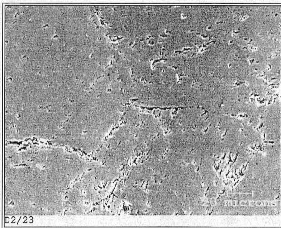
Figure 43. Marble D, unused. SE-image, 500x.
