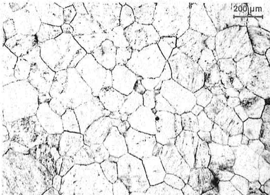
Figure 25. Microstructure of marble D. Unused. Plane-polarized light.
