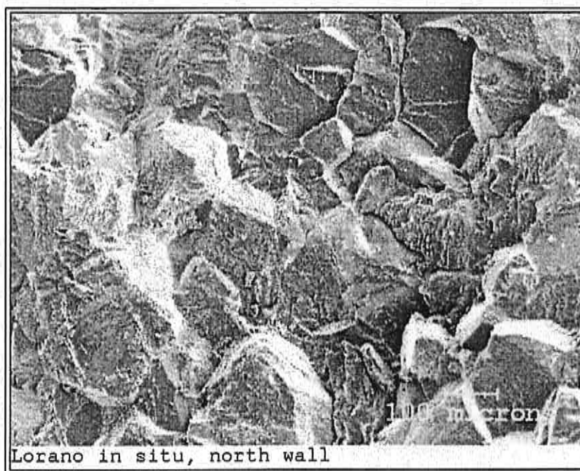
Figure 126. Marble from Finlandia Hall, north wall. SE-image of fractured surface, 100x.
