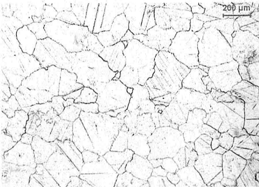
Figure 22. Microstructure of marble A. Unused. Plane-polarized light.
