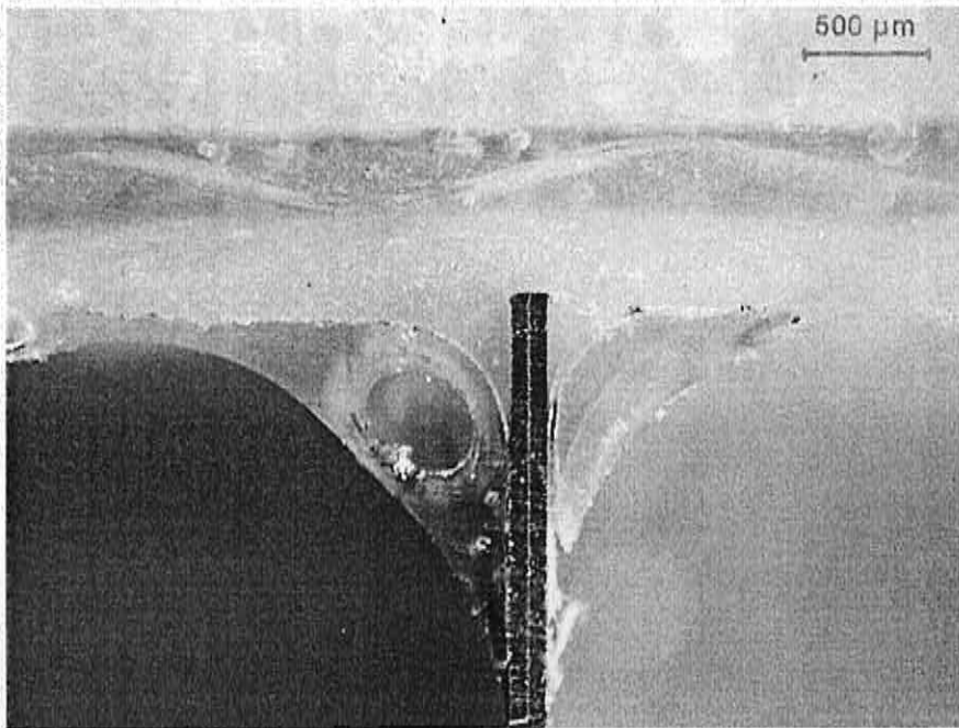
Figure 84. Microstructure of marble clad element H. 1.5 years on the test wall. Objective 2.5x, oblique illumination.
