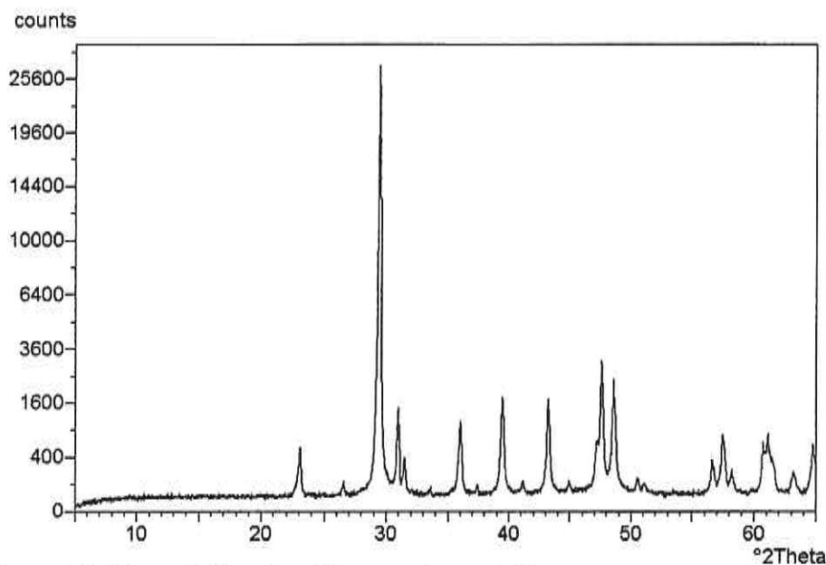
Figure 15. X-ray diffraction diagram of marble E.
