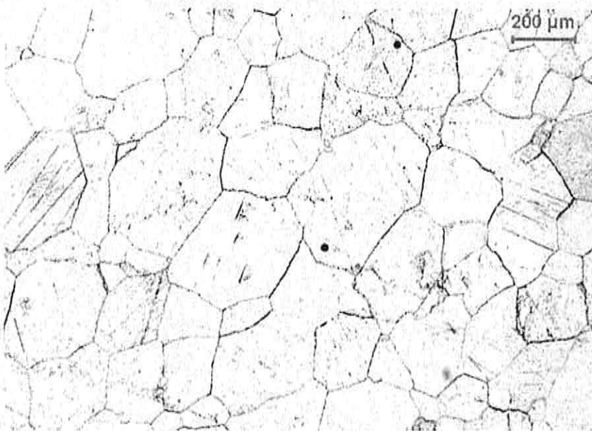
Figure 26. Microstructure of marble D. 1 year on the test wall. Plane-polarized light.
