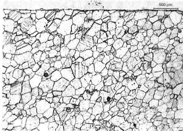
Figure 116. Microstructure of younger marble from case 2. Plane-polarized light.
