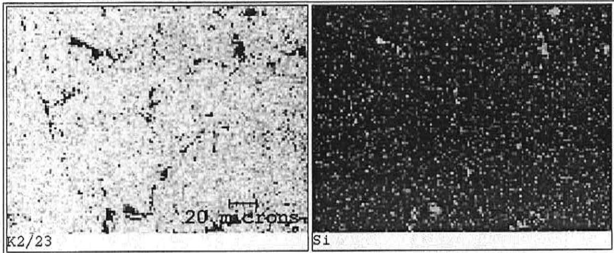
Figure 36. Marble K. Unused. BSE-image (500x, near the surface) and elementary dot map of silicon (Si).
