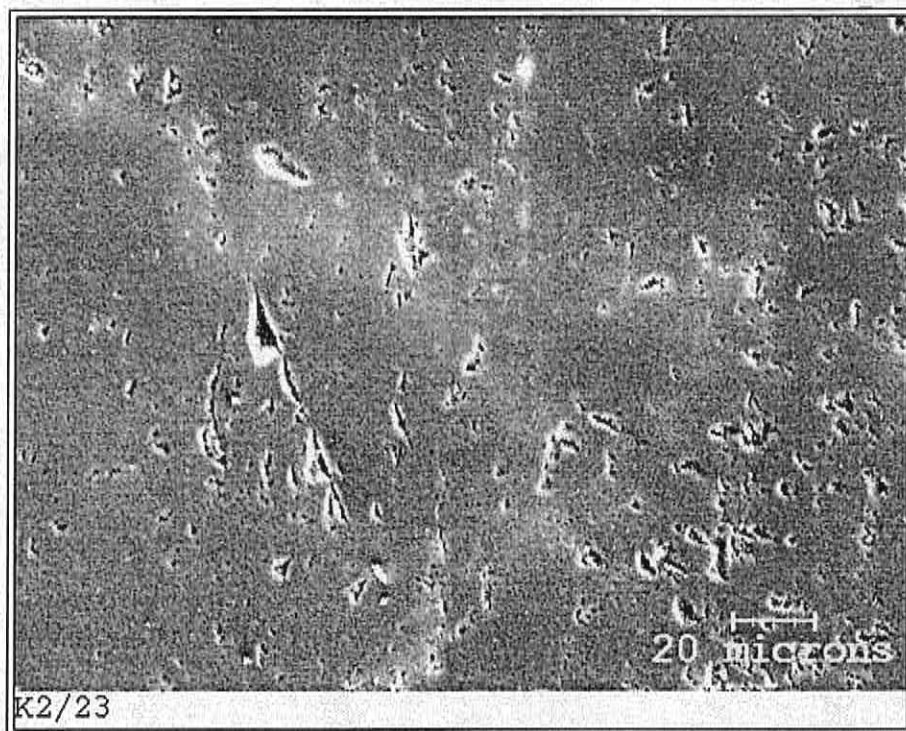
Figure 51. Marble K, unused. SE-image, 500x.
