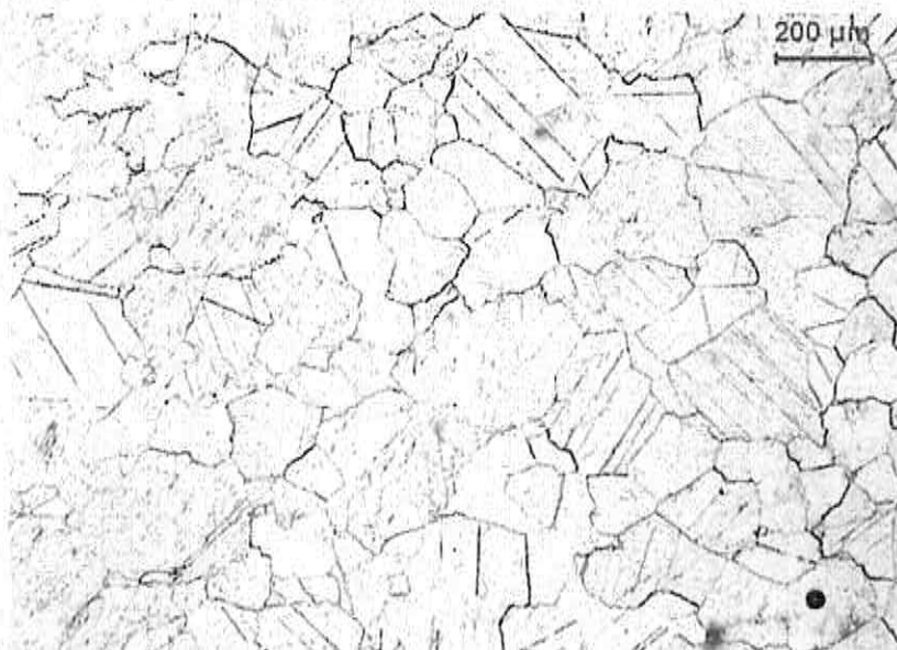
Figure 23. Microstructure of marble A. 1 year on the test wall. Plane-polarized light.
