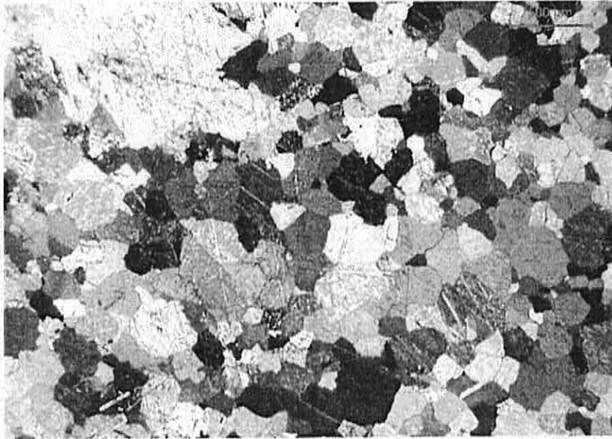
Figure 21. Microstructure of marble A. Unused. Cross-polarized light.
