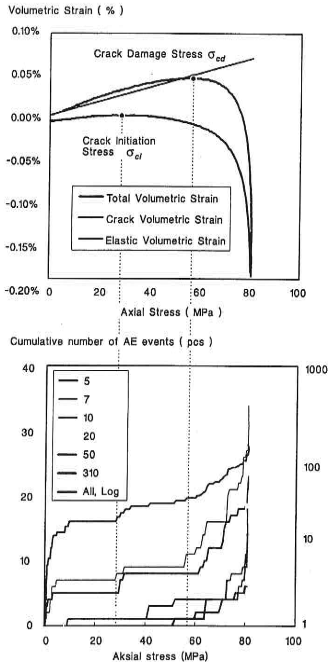
Figure 121. Comparison of typical strain and AE.
