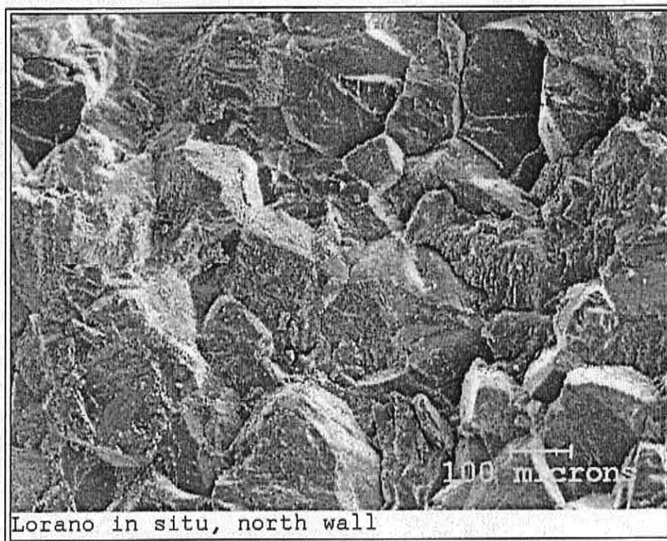
Figure 111. Marble from Finlandia Hall, north wall. SE-image of fractured surface, 100x.
