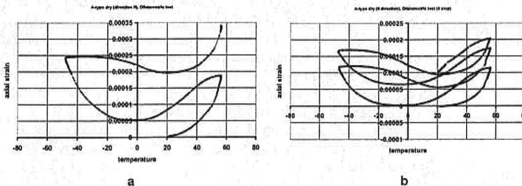
Figure 136. Average strain vs. temperature for A-type Marble. Same material as in Figure 135, but specimens rotated 90^{\circ} . Thermal cycles between t=+55^{\circ}\text{C} and t=-50^{\circ}\text{C} . Cycles n. 1-2 a and n. 4-5 b.
