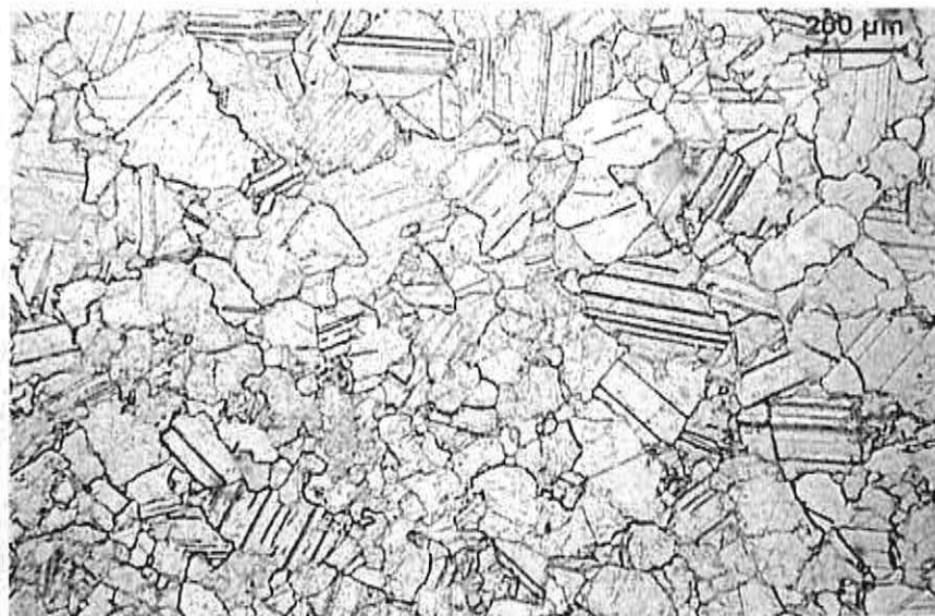
Figure 95. Microstructure of marble E(PA). 100 cycles in the climate chamber. Plane-polarised light.
