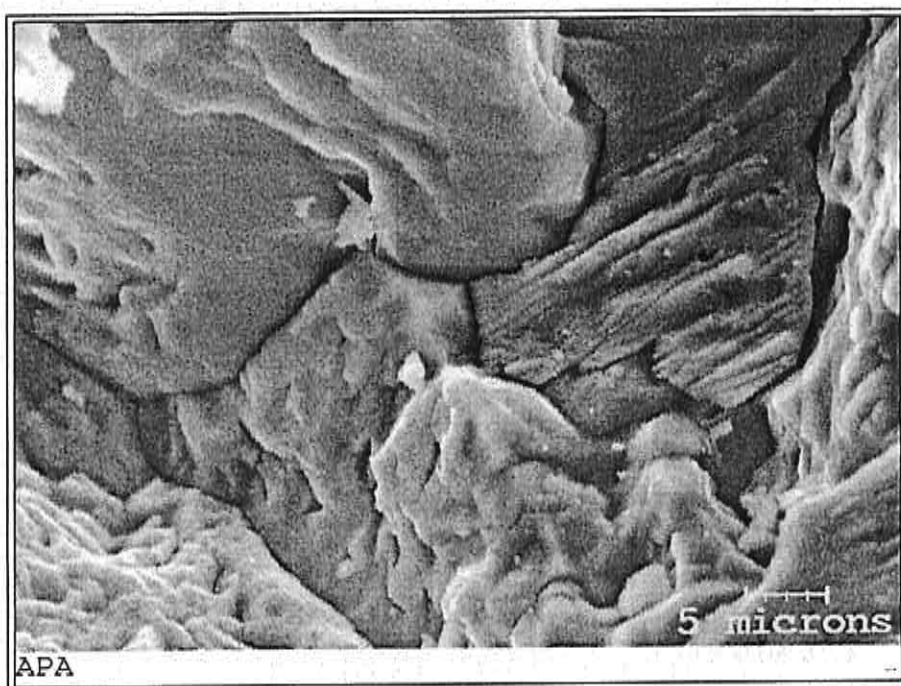
Figure 98. Marble E(PA), unused. SE-image of fractured surface, 2500x.
