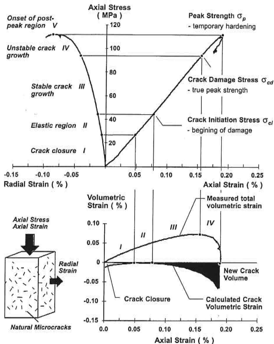
Figure 120. Determination of critical stress states \sigma_{cl} , \sigma_{cd} and \sigma_p (modified from Martin 1994).
