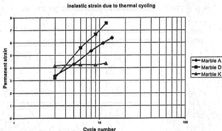
Figure 147. Permanent dilatation vs. number of cycles (semilogarithmic scale) for three different qualities of marble. Cycles performed between -50^{\circ}\text{C} and +55^{\circ}\text{C} .
