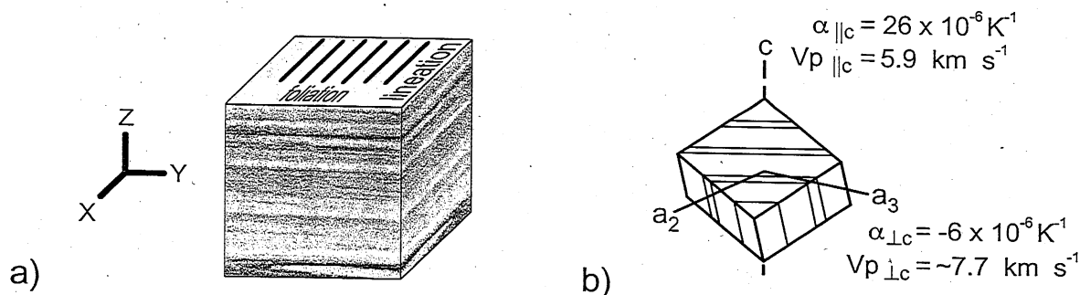
Fig. 1. (a) Reference coordinates with respect to foliation and lineation. (b) The calcite cleavage rhombohedron together with the values for thermal dilatation (Kleber 1959) and ultrasonic velocities (Dreyer 1974) in the directions of the c- and a-axes of the single crystal.
