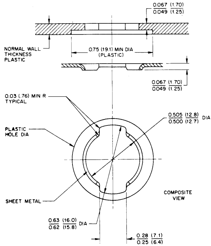
FIGURE A6—HOLE REQUIRED IN MOUNTING PLATE FOR 1/2 IN (12.7 MM) PRINTED CIRCUIT LAMP SOCKET WHEN BASE IN FLEXIBLE PLASTIC FILM
