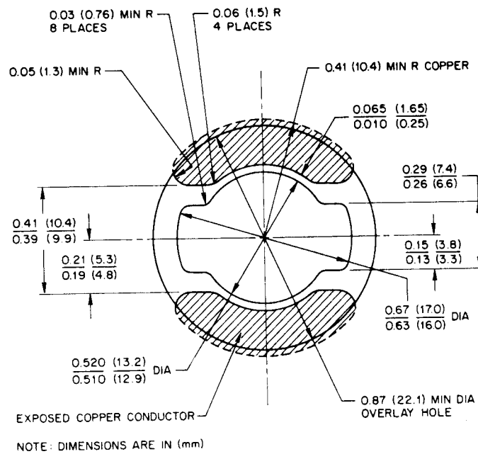
FIGURE A5—1/2 IN (12.7 MM) PRINTED CIRCUIT LAMP SOCKET HOLE STANDARD FOR FLEXIBLE PLASTIC FILM
