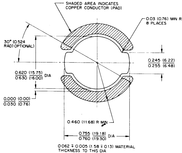
FIGURE A4—5/8 IN (15.9 MM) PRINTED CIRCUIT LAMP SOCKET HOLE STANDARD FOR RIGID PLASTIC OR PHENOLIC BASE
