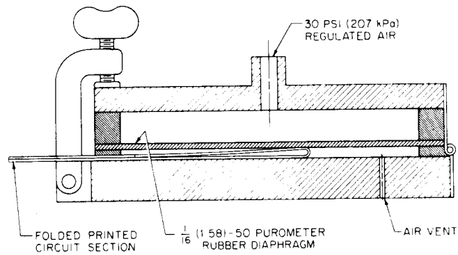
FIGURE A7—FOLD TESTER FIXTURE
