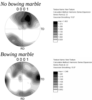
Figure 5. Pole figures of orientation densities in logarithmic scale, upper hemisphere, equal area projection: no bowing marble (top), bowling marble (bottom) based on stage scan of more than 6000 grains.
