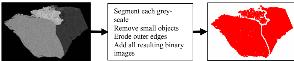
Figure 6-3. Binary image showing separated areas for every grey-level-region in a particle. By means of the separated areas in binary image, The Inca Feature software can perform individual EDS measurements for every grey-level (mineral grain) in one operation. (Figure: Torkjell Breivik).
