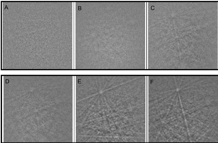
Figure 1. Diffraction patterns from quartz after increasing time of colloid silica polishing. A) 0 sec, B) 10 sec, C) 20 sec, D) 30 sec, E) 60 sec, F) 240 sec.
