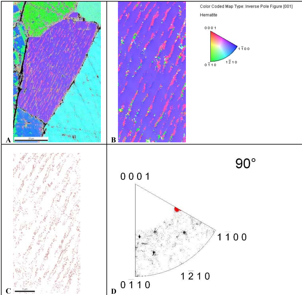
Figure 10. A) EBSD inverse pole figure map of hematite grain containing lamellas. B) Close up of grain from A. C) Twin boundaries. D) Inverse pole figure of axis of rotation at 90° misorientation. The red population shows the boundaries from C. Misorientation between parent and daughter is 90@<2 -2 0 1>.
