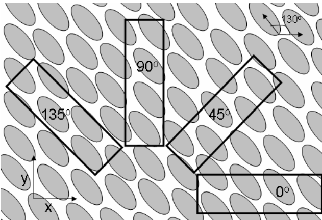
Figure 8. The orientation distribution displays a weak preferred 130^\circ orientation for the xy-plane of bowing marble. Elongation and orientation of the grains will therefore give rise to different numbers of grain boundaries along the longer dimension of the laboratory marble slabs when the slabs are cut in different directions. The 45^\circ slab will contain the highest number of grain boundaries along the longer dimension whereas the 135^\circ slab will contain the lowest number of grain boundaries.
