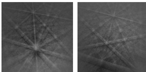
Figure 3. EBSD patterns from 2 orientations of calcite.
