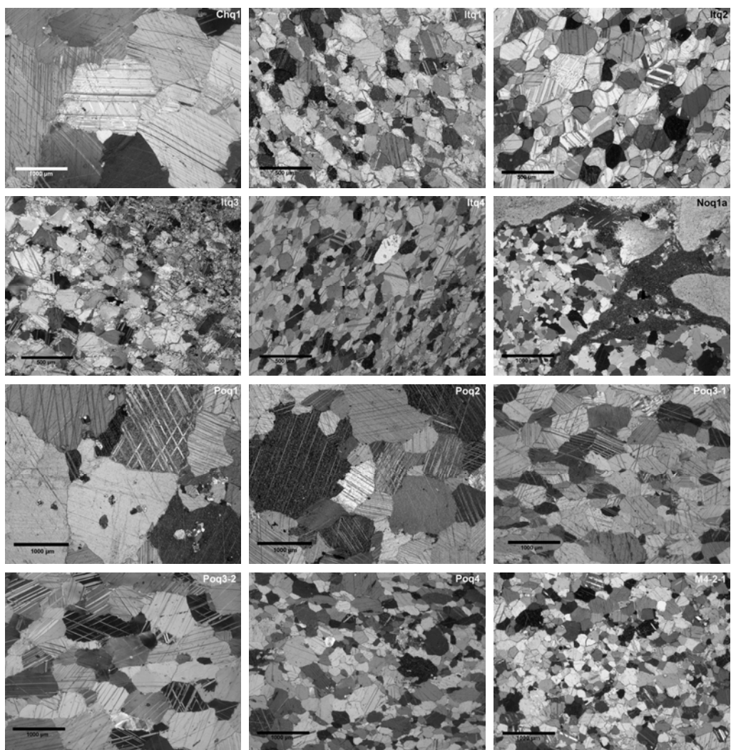
Figure 3. Microstructure of the investigated marbles. Scalebar is displayed in the lower left corner and sample code in the upper right corner.
