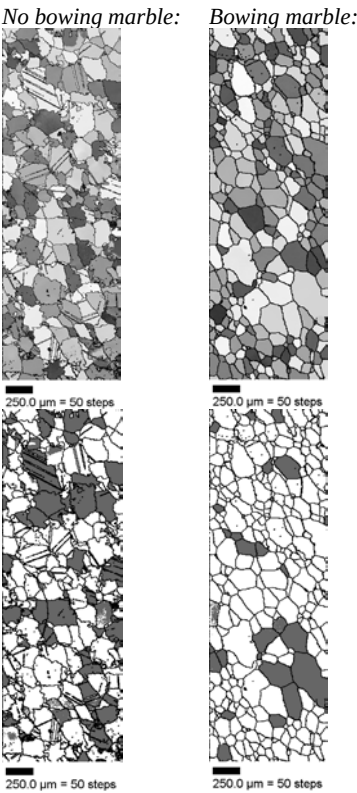
Figure 4. Inverse pole maps (top), grain boundary maps including grains with a preferred orientation (plotting in the dark maxima of the <0001> pole figures (bottom)).
