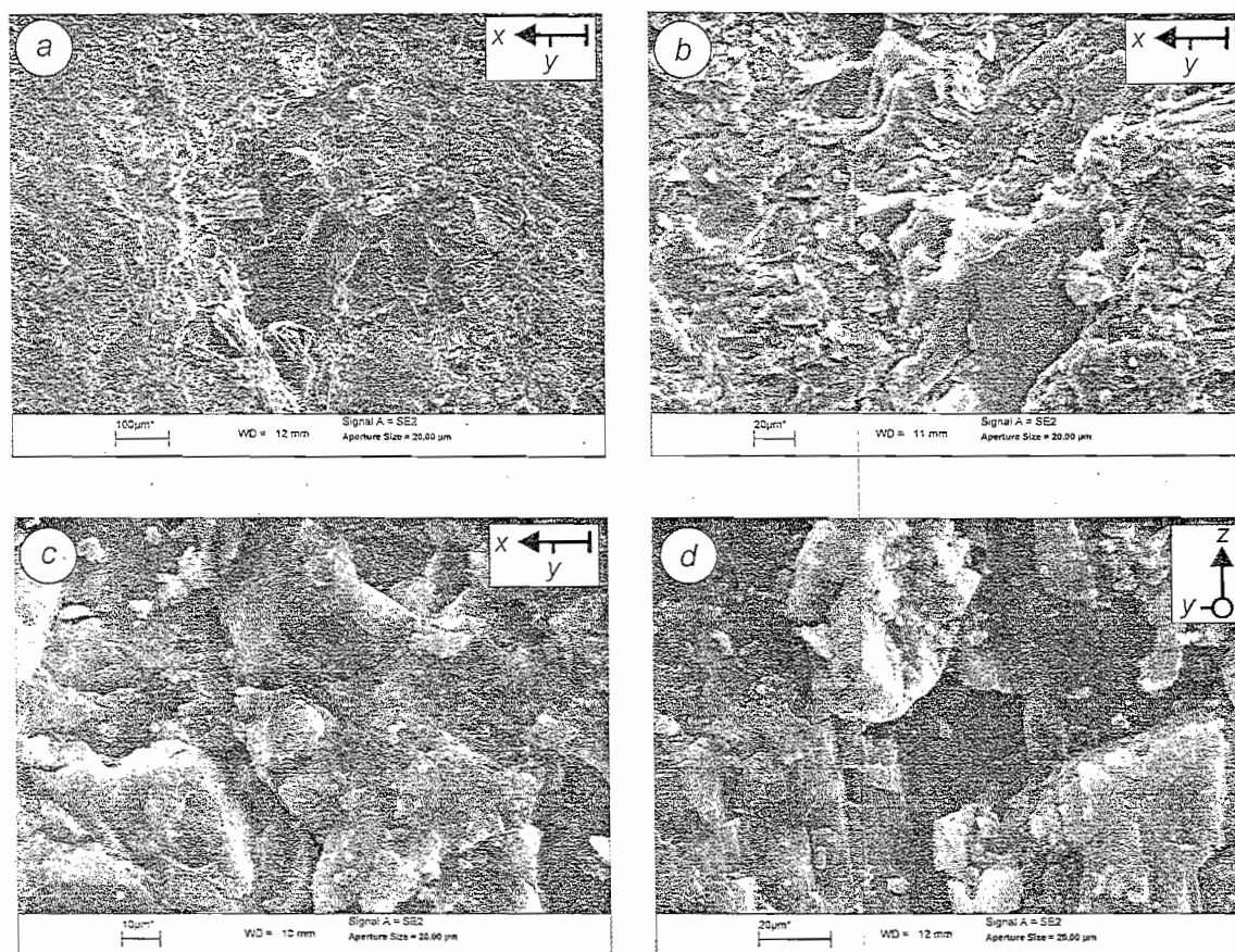
Fig. 15. Activated planes in Bohme test (abrasive test). Scanning electron micrographs; secondary electrons. (a, b) Activated (001) planes of muscovite. (c) Quartzitic area after the Bohme test. (d) Activated (001) and (010) planes in K-feldspar.
