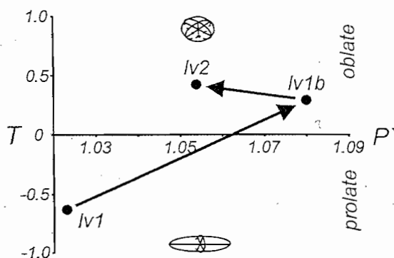
Fig. 7. P-T diagram after Jelinek (1981).
