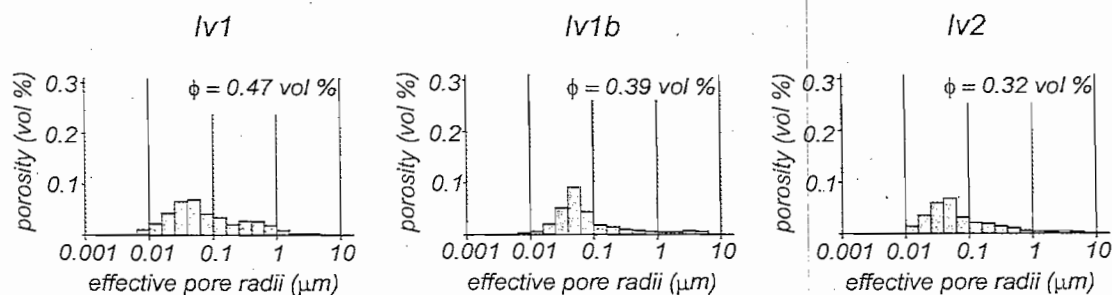
Fig. 4. Pore radii distribution. \Phi is total porosity.
