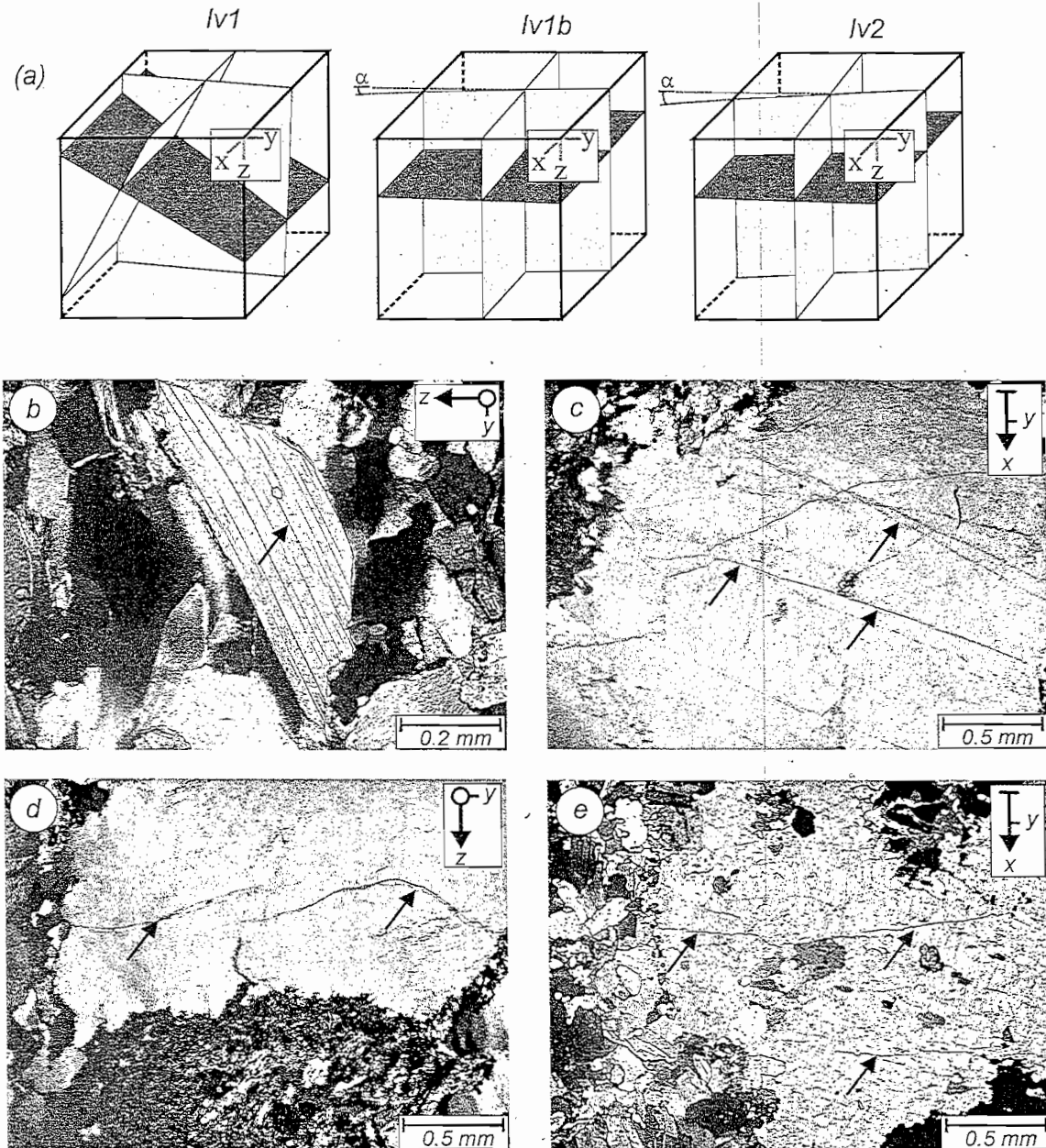
Fig. 8. Pre-existing microcracks. Optical micrographs; crossed polarizers (a) Orientation of microcrack systems in Iv1, Iv1b and Iv2; dark grey planes mark the preferred orientation of muscovite (001) cleavage planes. (b) Open cleavage cracks in muscovite; example marked by arrow (sample Iv1b). (c) Healed microcracks decorated with secondary fluid inclusions; examples marked by arrows (sample Iv1). (d) Mineralized microcracks in quartz marked by arrows (sample Iv1). (e) Open microcracks in K-feldspar; examples marked by arrows (sample Iv1b).
