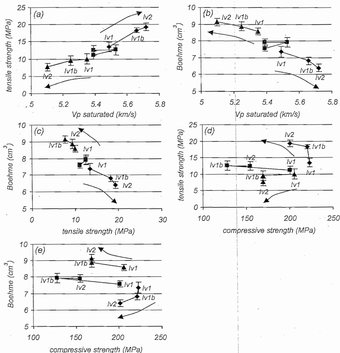
Fig. 17. Relations between mechanical and seismic parameters. The x-direction is marked by rhombes; y-direction marked by squares; z-direction marked by triangles; arrows display development of values due to progressive mylonitization. Experimental errors of compressive strength (d, e) see Table 4. For details see text.
