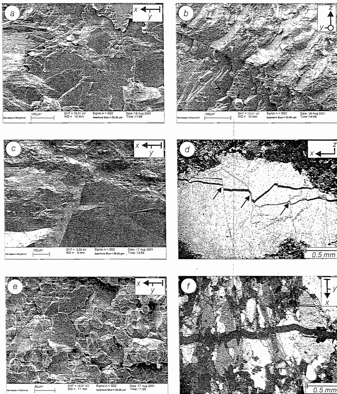
Fig. 10. Favourably activated planes in Brazilian test. Scanning electron micrographs; secondary electrons (a–c, e) and optical micrographs; crossed polarizers (d, f). (a) Activated (001) plane in muscovite. (b) Fracture of K-feldspar (baveno-twin); (001) and (010) cleavage planes activated. (c) Activated healed microcrack in quartz. (d) Activated healed microcracks in quartz marked by arrows. (e) Fracture pattern in microcrystalline quartzitic area. (f) Fracture plane filled by resin in sample Iv1b.
