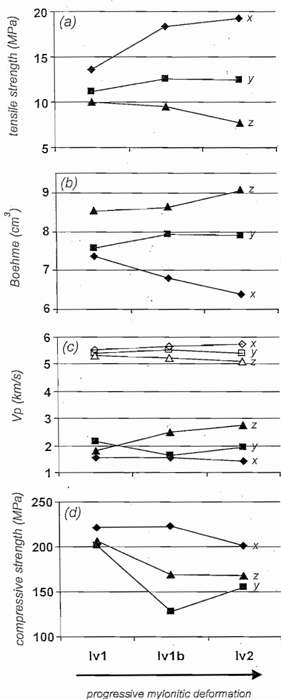
Fig. 16. Mechanical parameters and compressional wave velocities due to progressive mylonitization. The measured directions are indicated. (a) Tensile strength. (b) Abrasive strength (Boehme method); x-, y-, z-directions correspond to the planes perpendicular to the x-, y-, z-axes of the reference system. (c) Compressional wave velocities of water-saturated spherical samples (open symbols) and calculated \Delta Vp (bold symbols). (d) Compressive strength.
