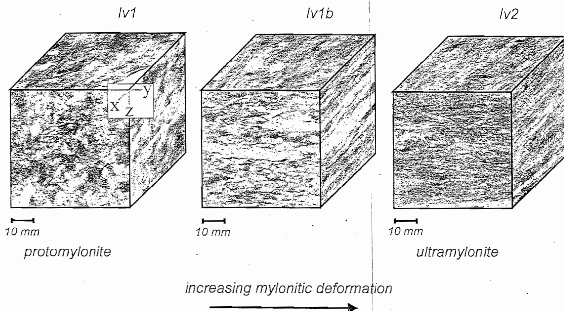
Fig. 2. Foliation development due to mylonitization. Scanned cubes. Dark layers are chlorite and clinozoisite/epidote enriched; bright layers are quartz and albite enriched.
