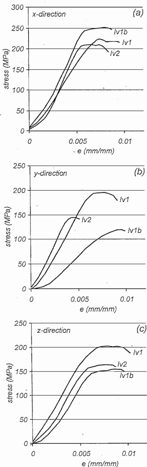
Fig. 13. Stress-strain curves derived by uniaxial compression test.
