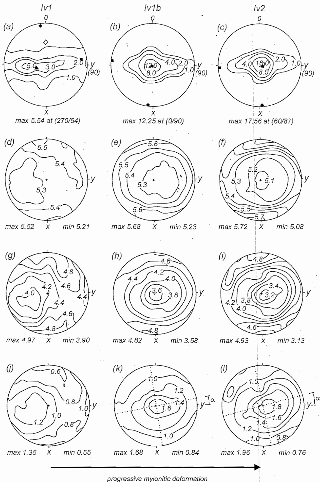
Fig. 6. Muscovite texture and compressional wave velocities. (a-c) Muscovite (001) poles in multiples of random distribution (220 grains per sample); main axis of AMS ellipsoid: K_{max} (rhombes); K_{int} (squares); K_{min} (triangles). (d-f) V_p ( \text{km s}^{-1} ) pattern of the water-saturated spherical specimens. (g-i) V_p ( \text{km s}^{-1} ) pattern of dry spherical samples. (j-l) Calculated \Delta V_p pattern ( V_p of saturated sample minus V_p of dry sample); dotted lines show estimated maxima of planes of microcrack systems excluding the muscovite cleavage planes. Estimates of V_p experimental error are \pm 50 \text{ m s}^{-1} .
