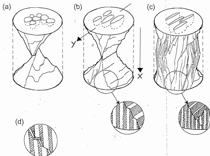
Fig. 11. Fracture pattern after uniaxial compression test. Samples cored and tested parallel to the x-direction. The x- and y-axes of the reference system are indicated in (b). (a) Iv1. (b) Iv1b. (c) Iv2. (d) Crack propagation during uniaxial compression test; arrows mark dislocation direction.
