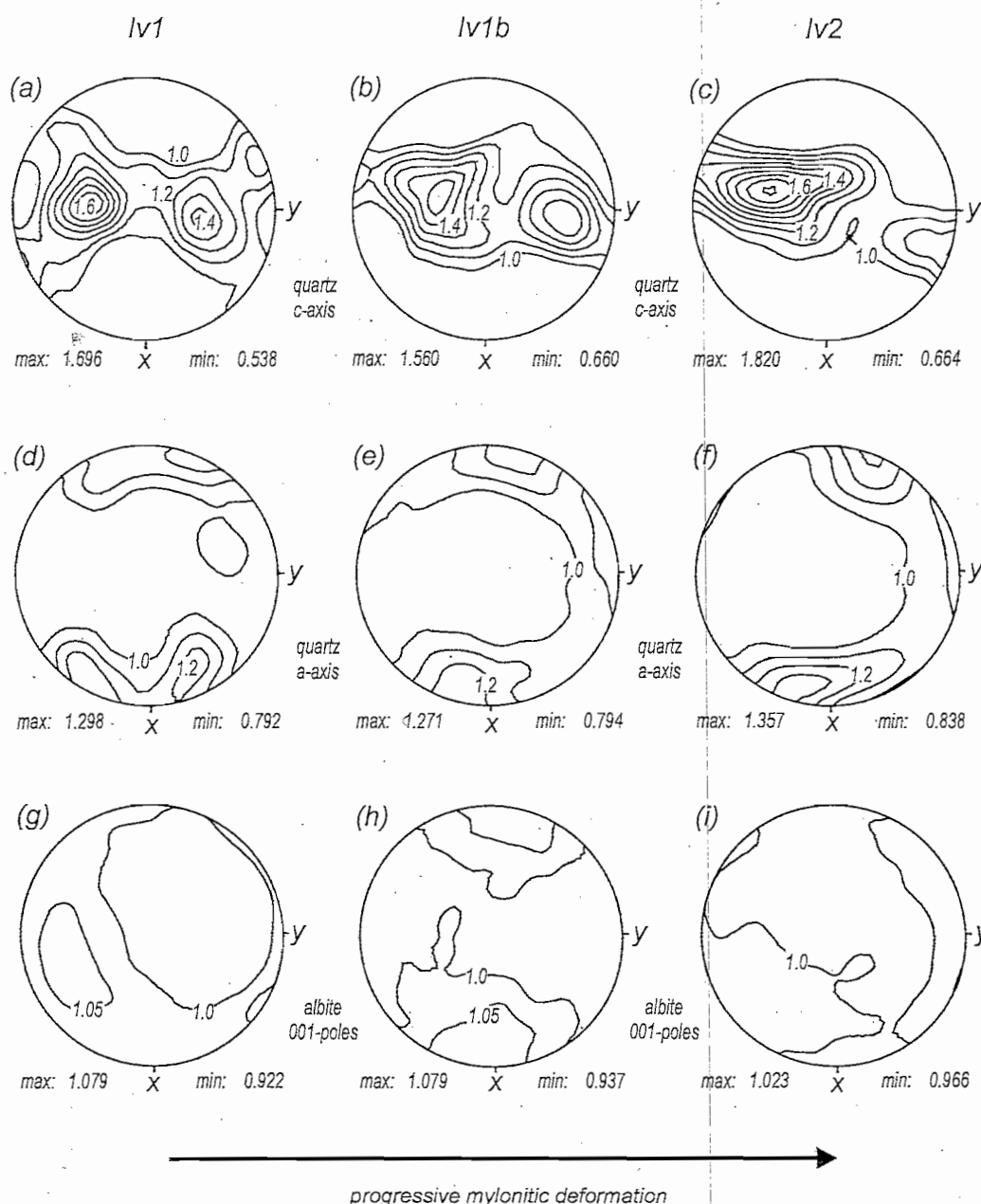
Fig. 5. Quartz and albite texture. Schmidt-net lower hemisphere; multiples of random distribution. (a-c) Distribution of quartz c-axis. (d-f) Distribution of quartz a-axis. (g-i) Distribution of albite (001) poles.
