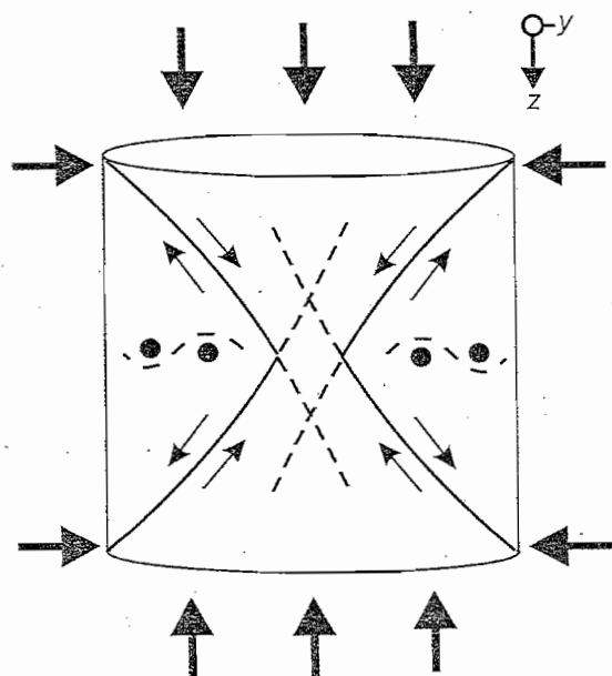
Fig. 12. Uniaxial compression test. Direction of sample load and forces at top and bottom of the sample (bold arrows); black lines mark planes of maximum shear stress; shear sense indicated by small arrows.
